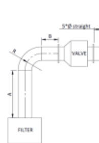
EQUIVALENT LENGTH CALCULATION (WITH ONE ELBOW) Only for Ø200-400
