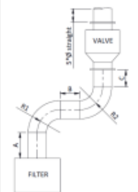
EQUIVALENT LENGTH CALCULATION (WITH TWO ELBOWS) Only for Ø200-400
